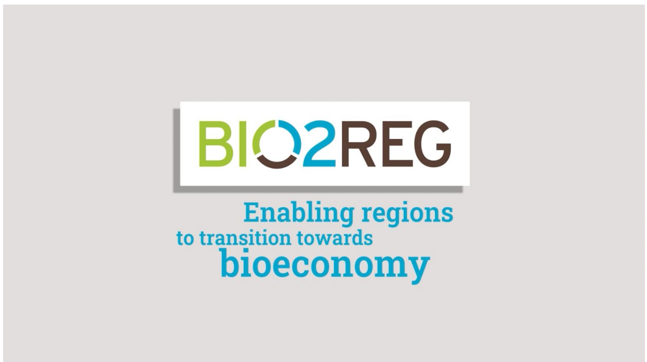
Figure 1: Introductory slide
