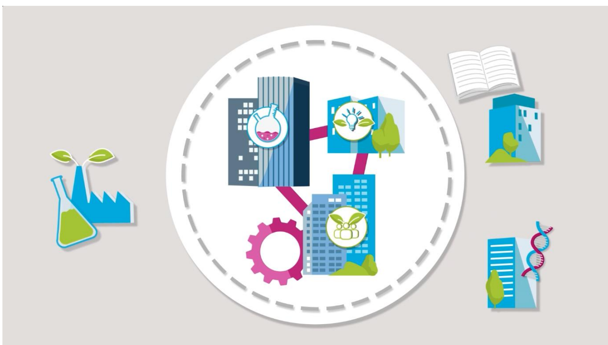
Figure 15: Video 4 animation
